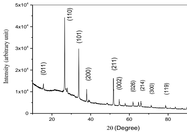
Figure 6 Reflection planes of La 2 O 3 doped SnO 2
